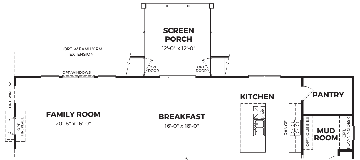
Partial First Floor at Opt. Screen Porch
