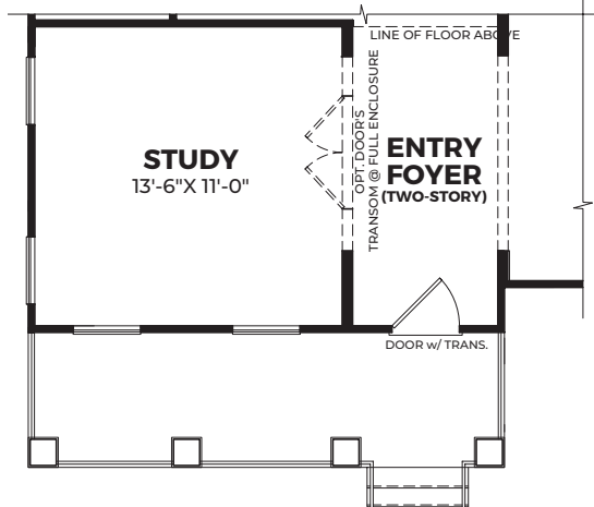
Partial First Floor at Craftsman
