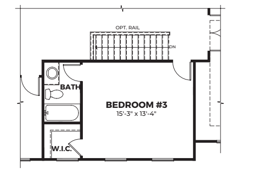
Partial Second Floor Plan w/ Opt. Bath #3
